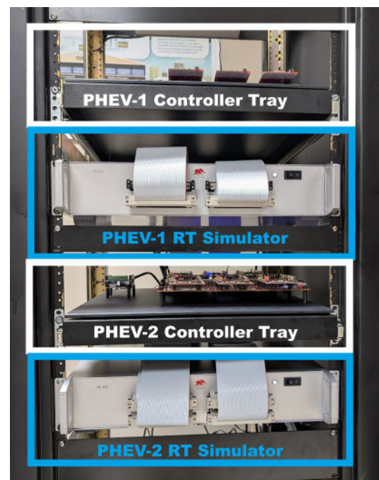
CHIL setup of the multi-PHEV system
