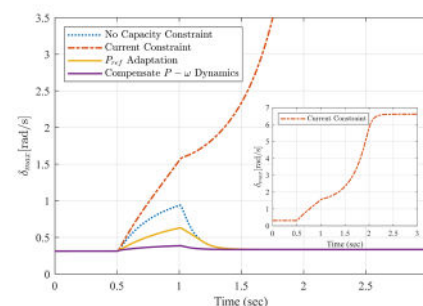
Maximum Power Angle Difference ( \delta ) between GFM inverters in a low-inertia network under various constraint and enhancement schemes
