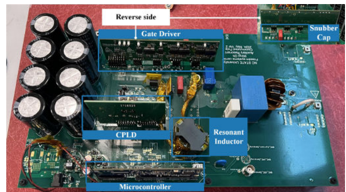
Hardware Prototype
