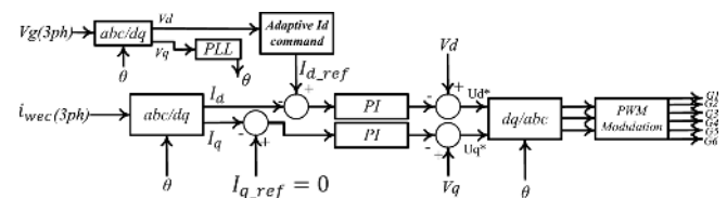
Adaptive Current Control Structure
