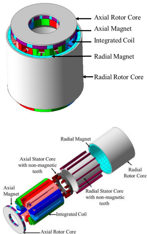
Design schematics of the Hybrid Flux Motor
