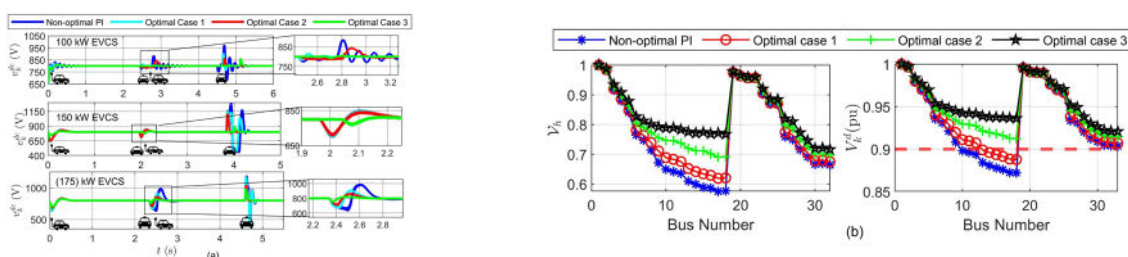
(a) DC bus voltage responses and (b) voltage stability indexes for PI-only and PI+LQR control across three optimal cases: 1) prioritizing small-signal stability, 2) prioritizing voltage stability, and 3) equal priority on both.
