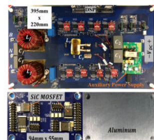
5kW hardware prototype
