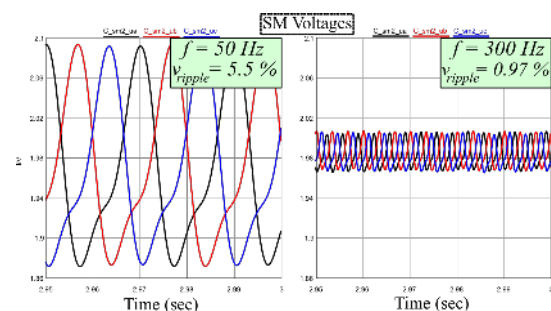
SM's Capacitor voltage ripple of MMC2 with 50 and 300 Hz
