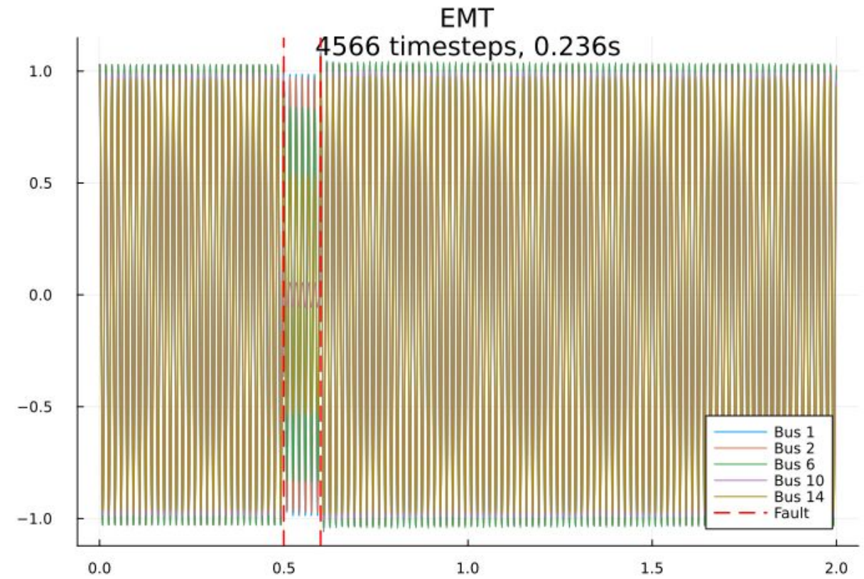
EMT vs Phasor Comparison - ieee14 - Bus 10 Fault (xf=0.01)
